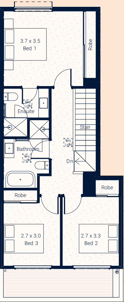
Second Floor
